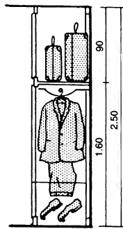
Section → 7
